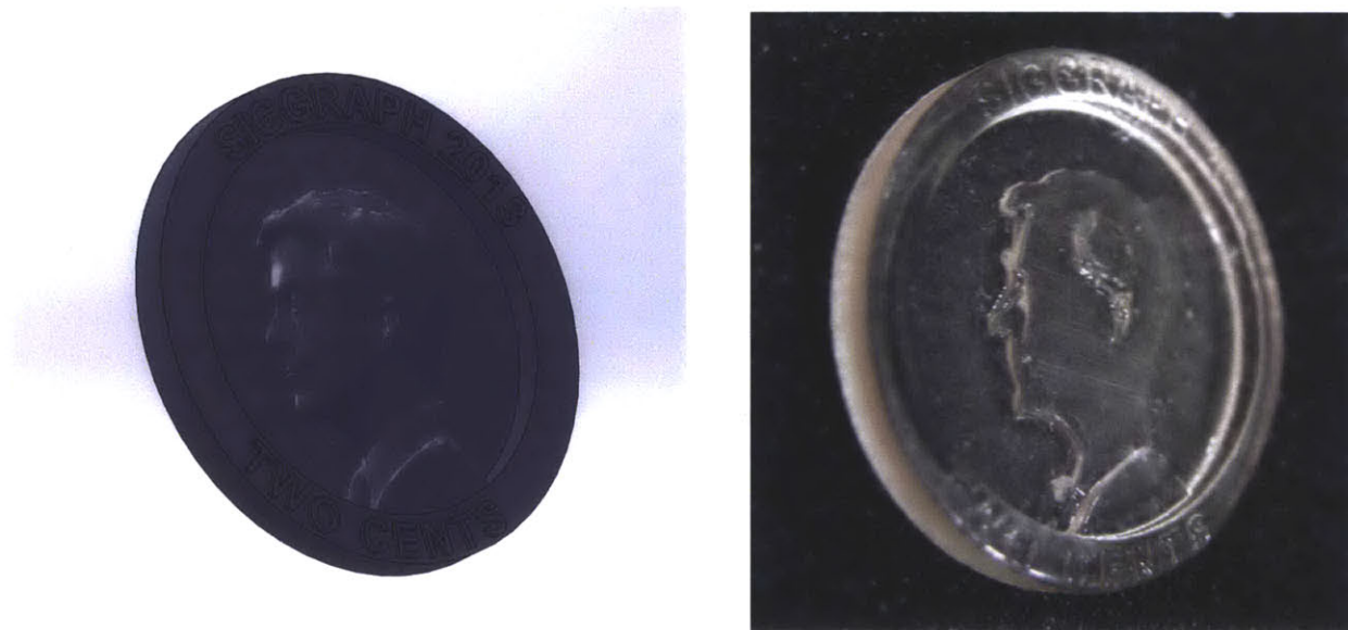
Figure 26: A test object as designed (left) and printed using the "E-20" polymer (right). The printed object measures approximately 25mm in diameter.
