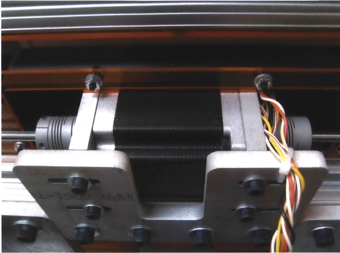
Figure 14: The double-shafted stepper motor used to actuate the Y-axis. Helical beam couplings are used to attach each end of the motor to its corresponding pulley drive shaft.
