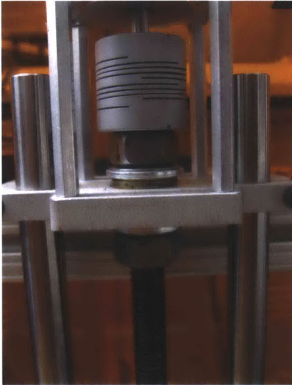
Figure 16: A close-up photo (left) and labeled diagram (right) of the top end of one of the Z-axis screw drives. The helical coupling compensates for misalignment between the lead screw and the stepper motor, while the needle thrust bearings support the weight of the platform.
