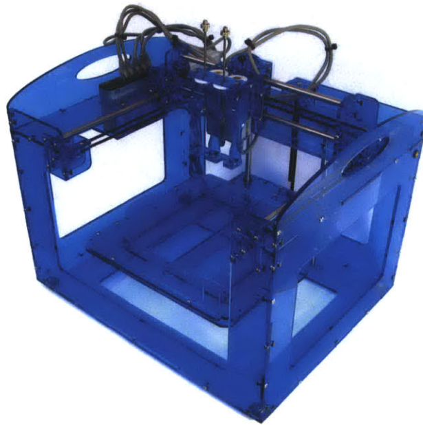
Figure 3: A Fab@Home Fabber Model 2. The printer is made primarily from laser-cut acrylic and features a closed-loop positioning system. Image from the Fab@Home Wiki [8].
