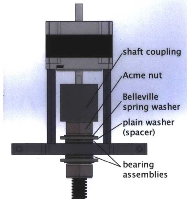
Figure 16: A close-up photo (left) and labeled diagram (right) of the top end of one of the Z-axis screw drives. The helical coupling compensates for misalignment between the lead screw and the stepper motor, while the needle thrust bearings support the weight of the platform.
