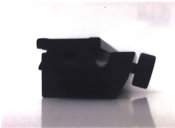
Figure 18: The optical rail (top) and carrier (bottom). The rail is attached to the underside of the carriage, and the carriers are attached to the modules. This allows the modules to be attached and removed easily by adjusting the thumbscrew.
