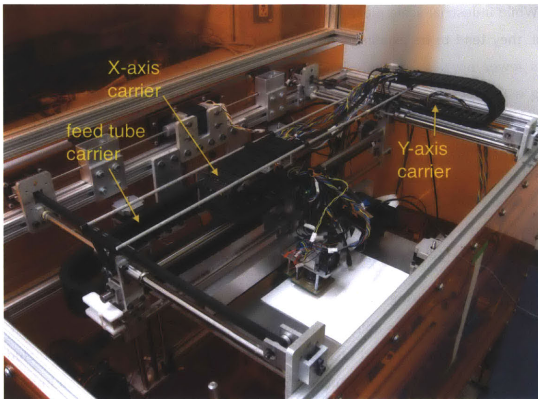
Figure 21: The three cable carriers in the printer. Cable carriers allow pipes and wires to be routed to the carriage in an orderly way without risk of entanglement or fatigue due to bending.
