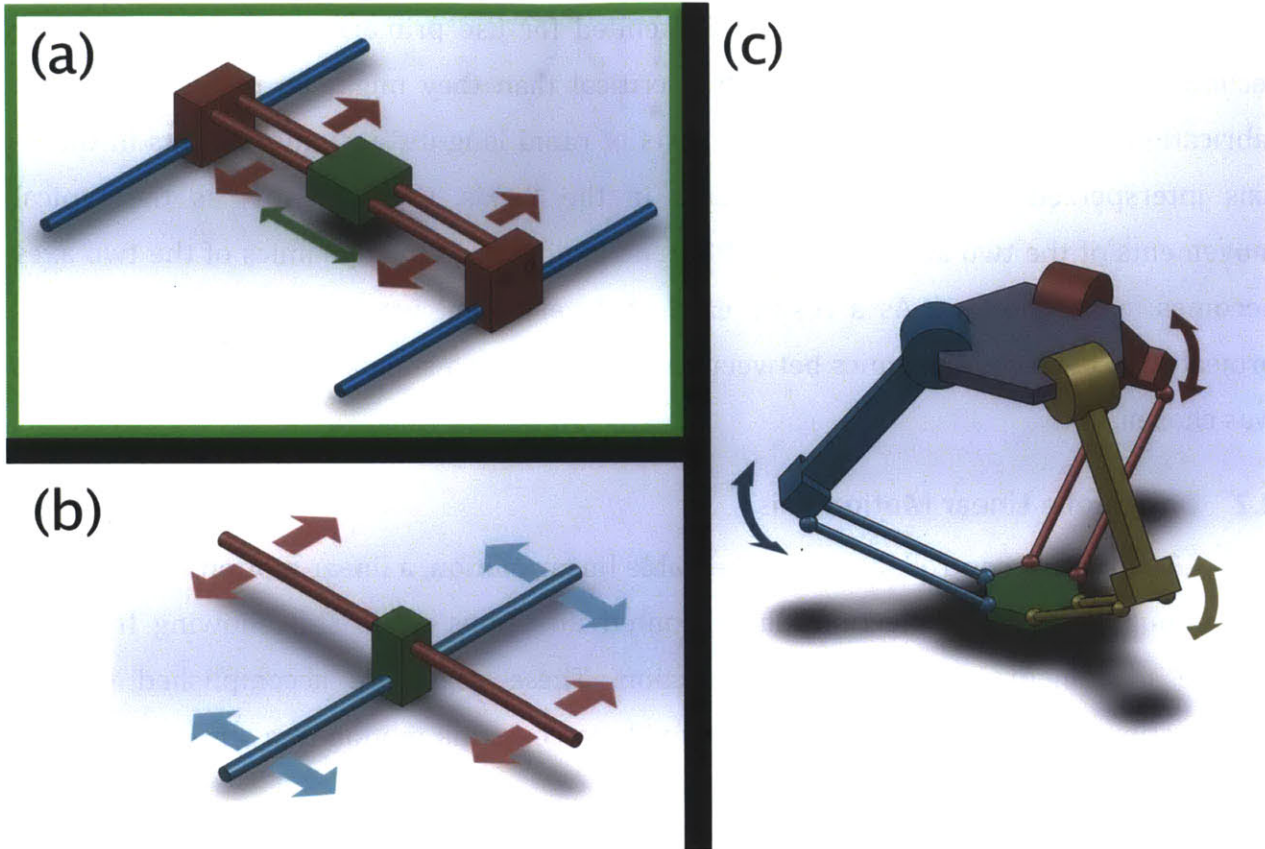
Figure 5: A series axes arrangement (a), a crossed axes arrangement (b), and a delta robot configuration (c). In each figure, the carriage being moved is shown in green. While the crossed axes and delta arrangements have superior dynamics, option (a) was eventually chosen for ease of development and increased carriage mounting space.
