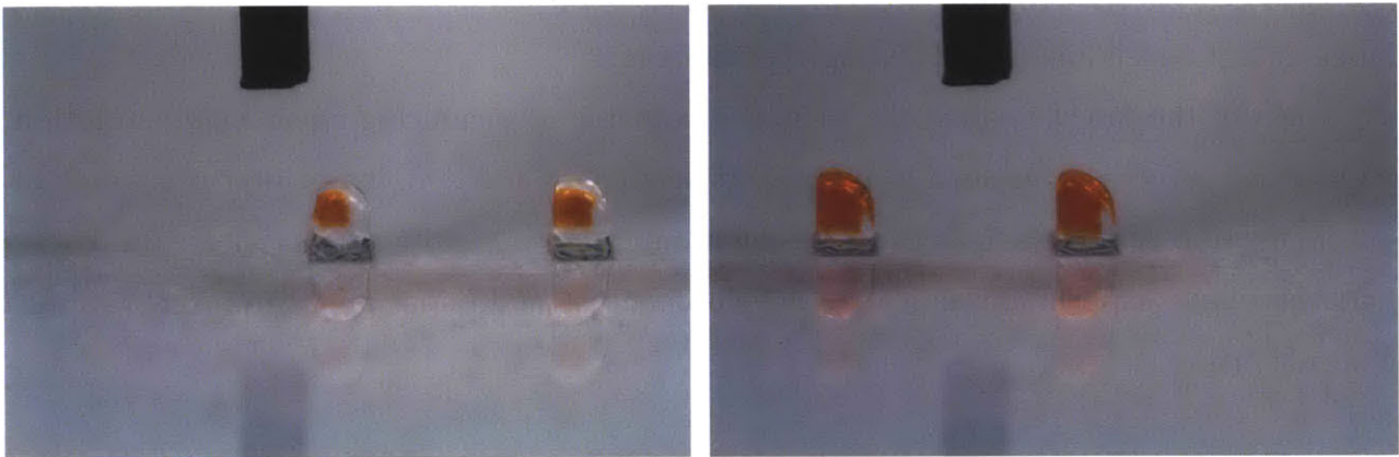
Figure 28: Photos showing the leftmost (left) and rightmost (right) multi-material dots from Figure 27 . The distortion in shape increases with the proportion of colored material.
