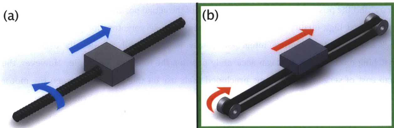
Figure 7: A screw drive (a) and a belt drive (b) were considered as transmission mechanisms. Option (b) was selected because the responsiveness of the belt drive was considered more important than the stiffness of the screw drive.
