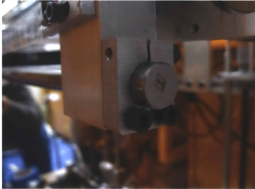
Figure 11: One of four end clamps of the X-axis guide rods. The clamps firmly secure the guide rods and prevent them from shifting axially.
