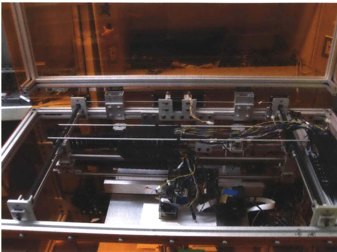
Figure 9: A view inside the printer, showing the X- and Y-axes.
