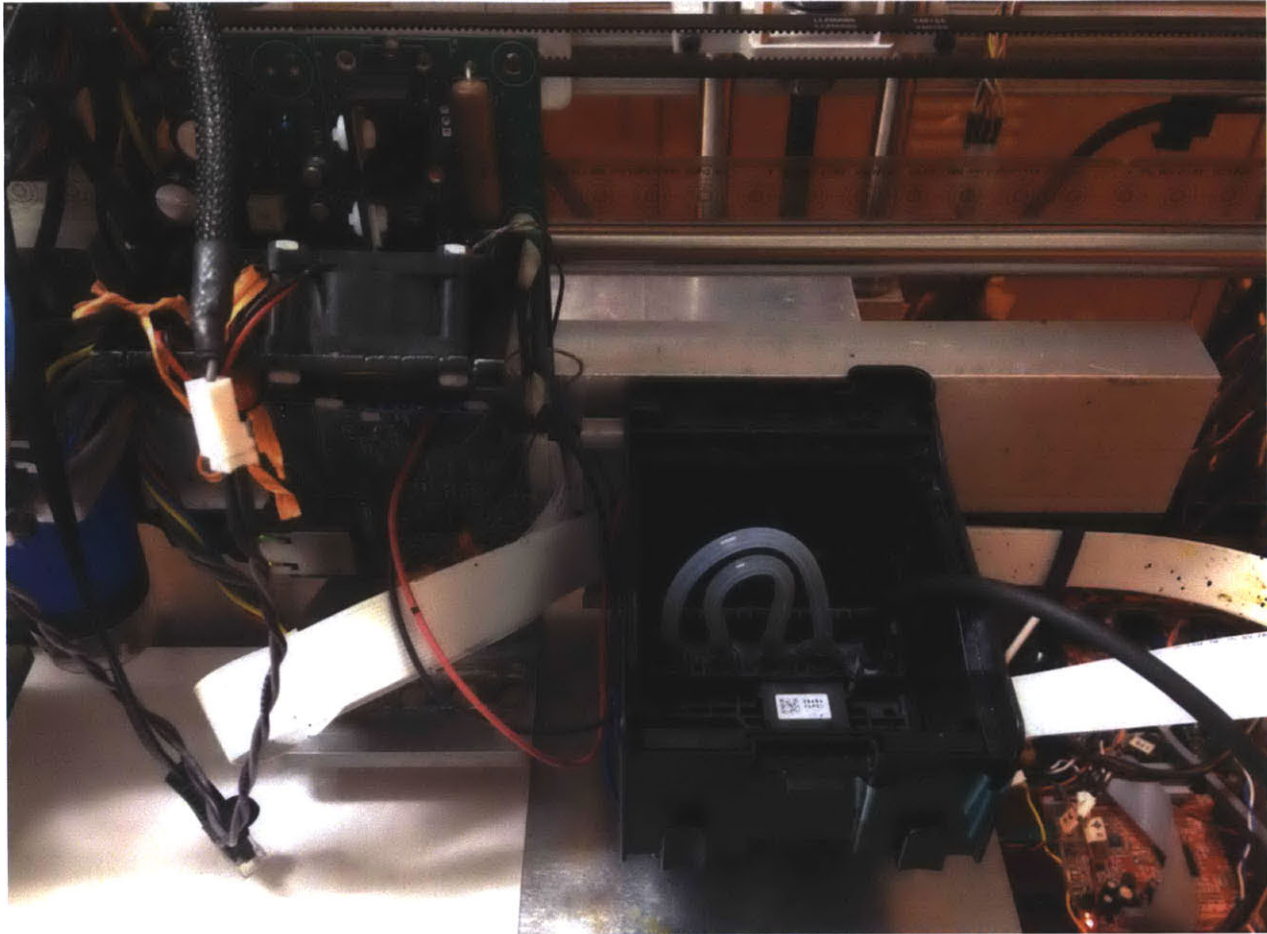
Figure 19: Two modules on the printer. The optical rail is attached to the underside of the aluminum box beam behind the module.
