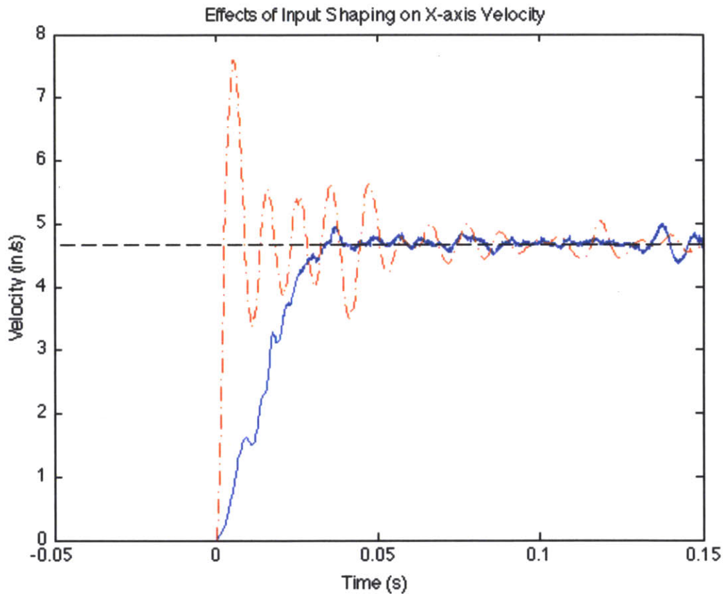
Figure 24: A comparison between the velocity of the X-axis without the ramping profile (red \cdot- line) and with it (blue solid line). The black dashed line shows the target speed of 4.6752 in/s (10000 \mu steps/s). During these experiments, the position of the carriage was recorded using the X-axis encoder and used to calculate the carriage's velocity. The resulting velocity values have been smoothed with a moving average filter with span 10.
