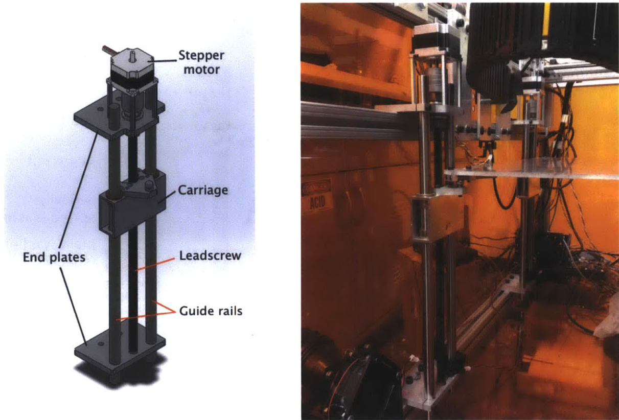
Figure 15: A CAD model (left) and photo (right) of a single screw-drive unit from the Z-axis. The motor at the top a leadscrew, which translates the carriage up and down. The screw drive mechanism is preloaded by the weight of the platform.
