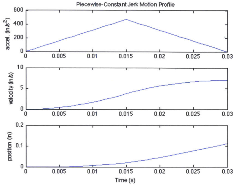
Figure 23: Acceleration, velocity, and position as a function of time using a piecewise-constant jerk profile, which linearly increases the system’s acceleration to a maximum value then decreases it again.
