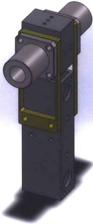
Figure 13: A CAD model of one end of the X-axis (left), showing the flexures (highlighted in yellow), and a photo of the flexures on the actual printer (right). The flexures were cut from aluminum sheet on the waterjet and allow the Y-axis bearings to shift laterally to compensate for misalignment and thermal expansion, while still supporting the weight of the X-axis.
