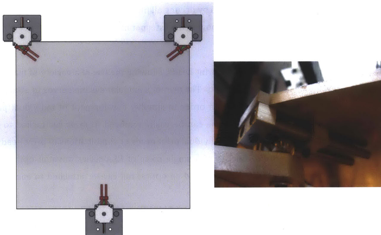
Figure 17: A top-down diagram of the build platform (left), along with a photo of the ball-and-shafts coupling mechanism (right). The diagram shows the the paired shafts (red) and precision balls (green) that form the kinematic coupling that joins the platform and the screw drive units. The platform has been made transparent in this image for ease of understanding.
