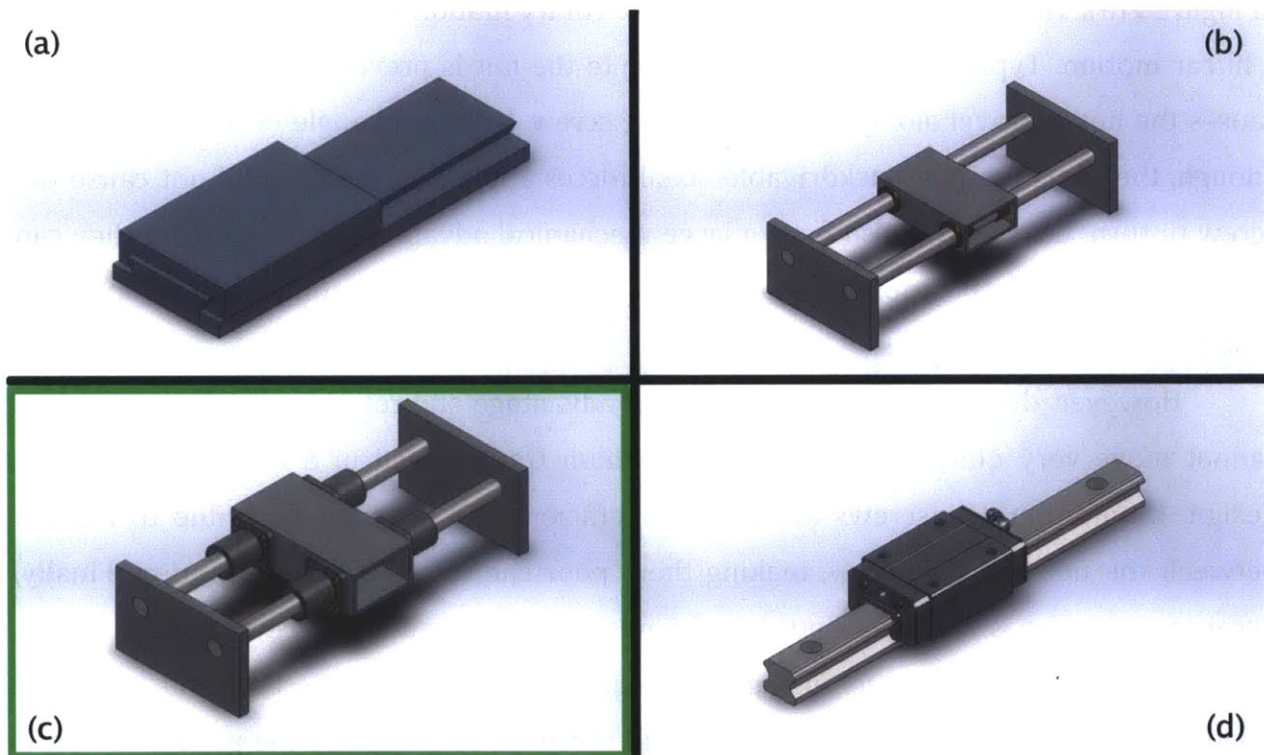
Figure 6: Dovetail rail (a), twin rails with bushings (b), twin rails with linear bearings (c), and linear motion rail (d), the four choices considered for linear guides on the printer. Option (c) was selected for its balance between cost, rigidity, and smoothness of motion.
