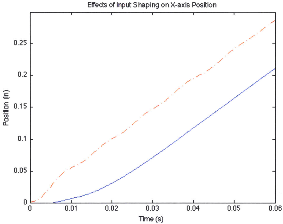
Figure 25: A comparison between the movement of the X-axis without the ramping profile (red \cdot- line) and with it (blue solid line).
