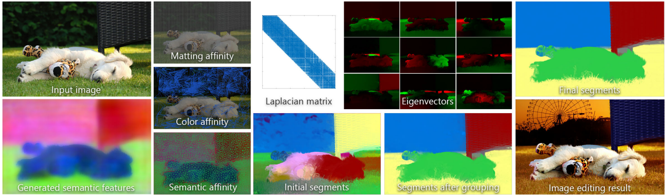
Fig. 2. For an input image, we generate per-pixel hyperdimensional semantic feature vectors and define a graph using the texture and semantic information. The graph is constructed such that the corresponding Laplacian matrix and its eigenvectors reveal the semantic objects and the soft transitions between them. We use the eigenvectors to create a set of preliminary soft segments and combine them to get semantically meaningful segments. Finally, we refine the soft segments so that they can be used for targeted image editing tasks.
