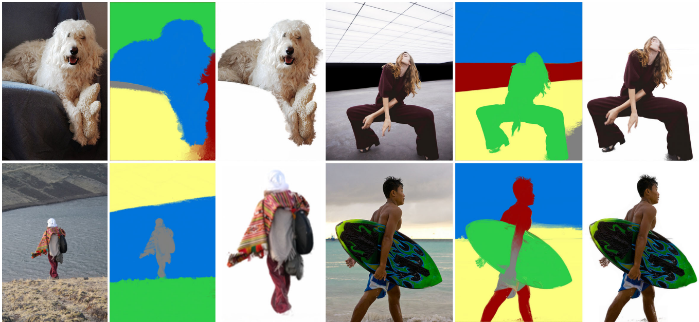
Fig. 1. We propose a method that can generate soft segments, i.e. layers that represent the semantically meaningful regions as well as the soft transitions between them, automatically by fusing high-level and low-level image features in a single graph structure. The semantic soft segments, visualized by assigning each segment a solid color, can be used as masks for targeted image editing tasks, or selected layers can be used for compositing after layer color estimation.
