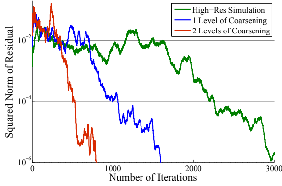
Figure 14: Comparison of CG iterations on high-resolution and coarsened meshes of the George-bone example. The squared residual is measured as \|\mathbf{K}\mathbf{x} - \mathbf{f}\|^2 . We observe that CG converges much faster on coarse meshes.
