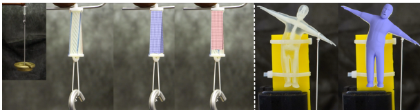
Figure 18: A comparison of DDFEM (2 levels of coarsening) to real world deformations of 3D printed, multi-material designs. DDFEM captures the twisting behavior of an anisotropic bar much more accurately than Naïve Coarsening . Similarly DDFEM accurately predicts the deformation of our heterogeneous George character.
